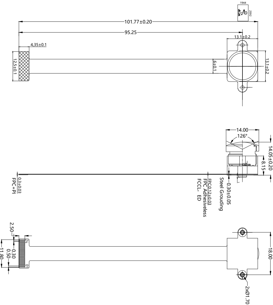
TOP VIEW
